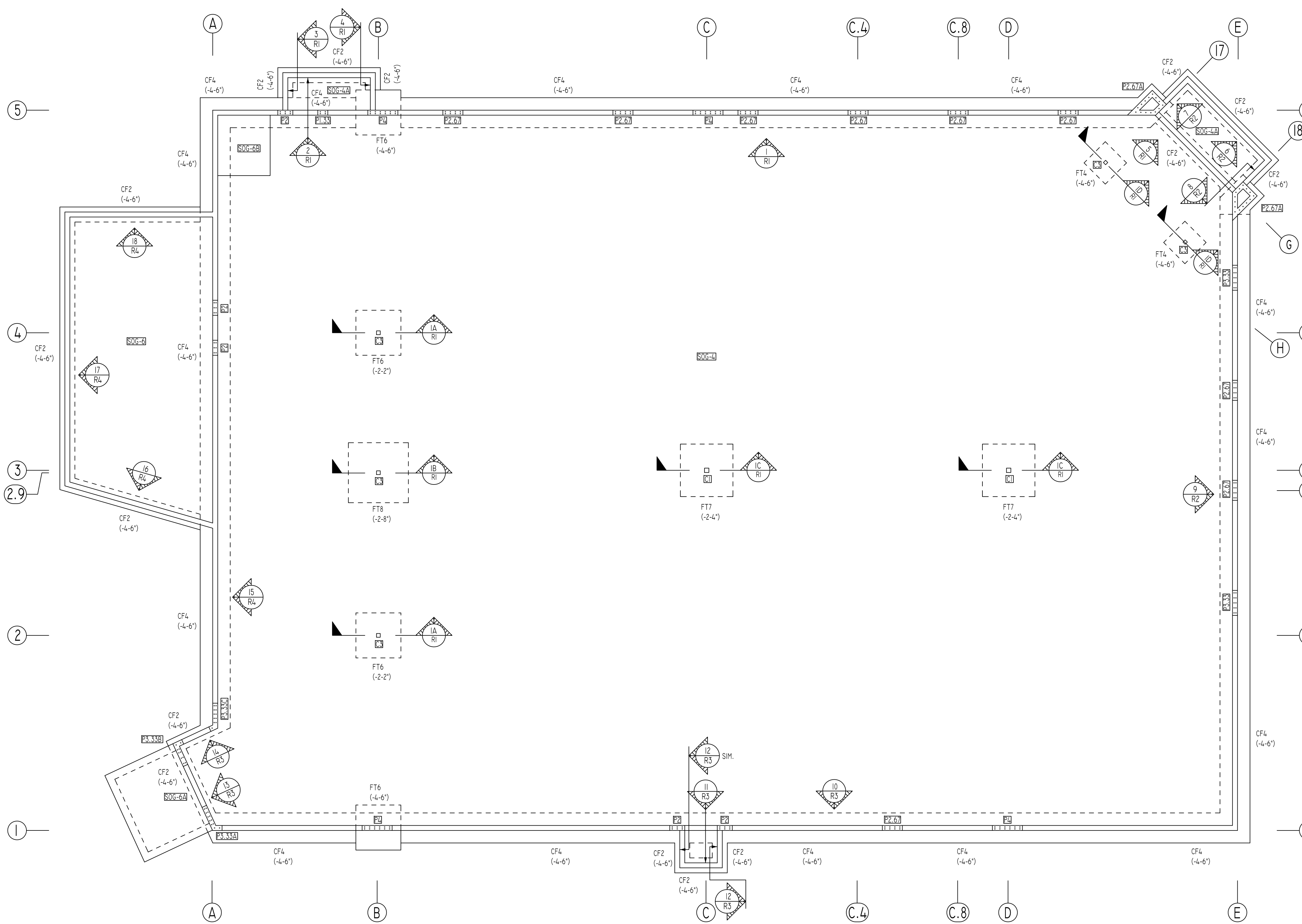
FOUNDATION PLAN SCALE - 1/8"=1'-0" REF. SI, S2, S4 & S5
