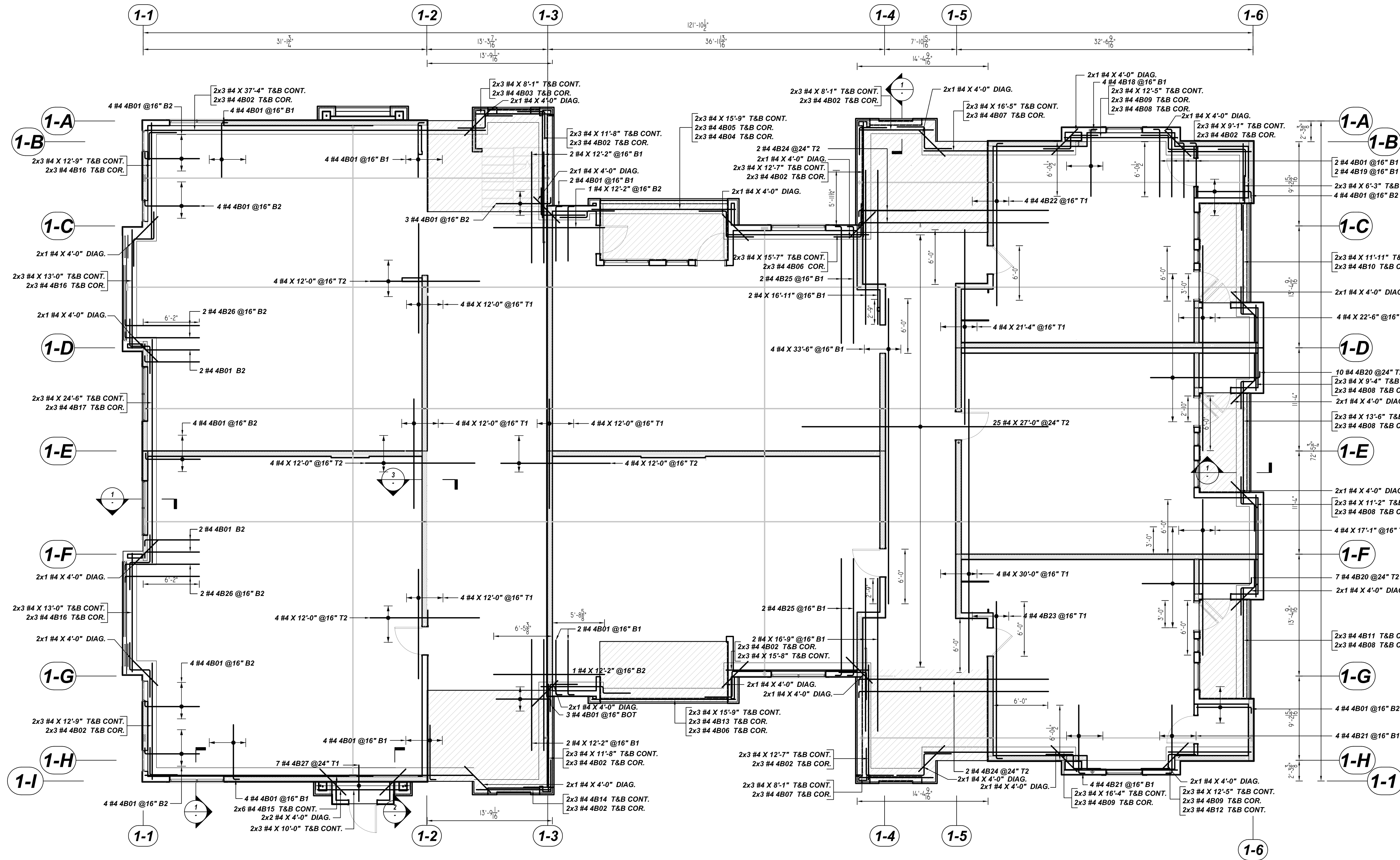
BUILDING 1 FOUNDATION REINFORCEMENT DETAILS REF: S2.11 (DT.07/27/22) SCALE: 1/8\"/>
